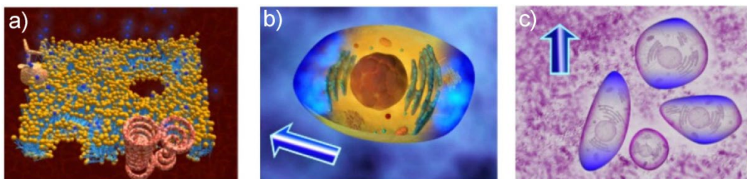
Figure 1: Introduction of small molecules (blue molecules) through a cell membrane (a) into an electroporated cell (b) and into the successfully electroporated cells within an exposed tissue (c) (Čorović et al., 2009).
