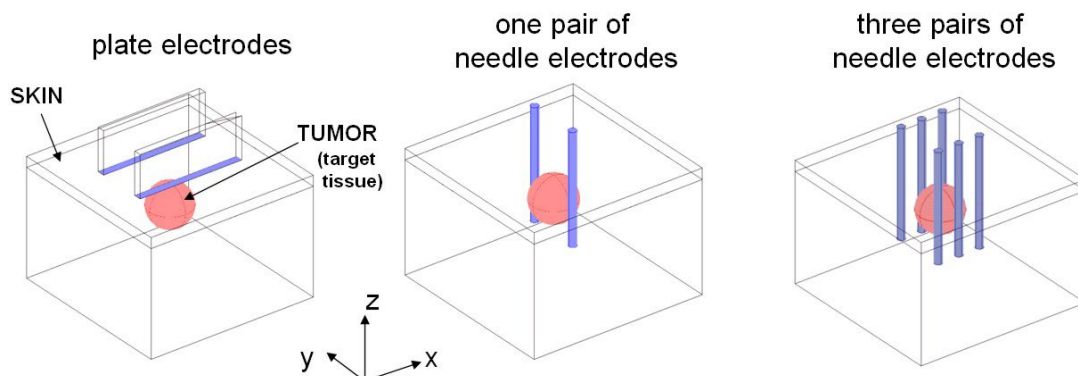
Figure 2: Plate electrodes vs. needle electrodes with respect to the target tissue (e.g. tumor tissue).
